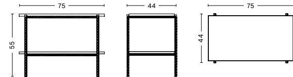
REBAR SIDE TABLE | RECTANGULAR Length 75 cm Width 44 cm Height 55 cm Weight 29,7 kg
