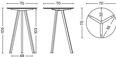
CPH 20 HIGH TABLE Ø70 X H105 Diameter 70 cm Height 105 cm Weight 10 kg
