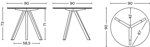
CPH 20 TABLE Ø90 X H73 Diameter 90 cm Height 73 cm Weight 17,5 kg
