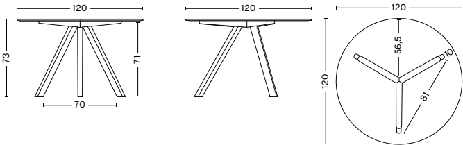
CPH 20 TABLE Ø120 X H73 Diameter 120 cm Height 73 cm Weight 25,3 kg
