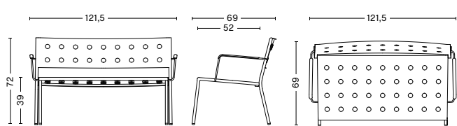
BALCONY LOUNGE BENCH W ARM Width 121,5 cm Depth 69 cm Height 72 cm Seat height 39 cm
