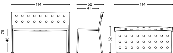
BALCONY DINING BENCH Width 114 cm Depth 52 cm Height 79 cm Seat height 46 cm
