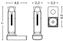
FIXATION BRACKET FOR BENCHES Width 4,5 cm Depth 2,2 cm Height 7 cm
