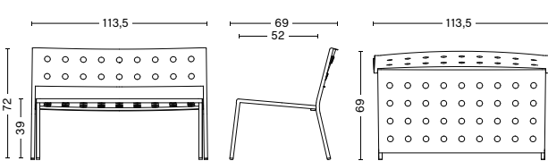
BALCONY LOUNGE BENCH Width 113,5 cm Depth 69 cm Height 72 cm Seat height 39 cm
