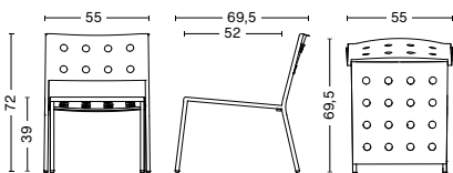
BALCONY LOUNGE CHAIR Width 55 cm Depth 69,5 cm Height 72 cm Seat height 39 cm Seat depth 52 cm
