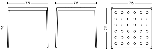
BALCONY TABLE Length 75 cm Width 76 cm Heigth 74 cm
