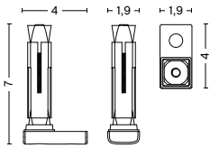
FIXATION BRACKET FOR CHAIRS, BAR STOOLS AND STOOLS Width 4 cm Depth 1,9 cm Height 7 cm
