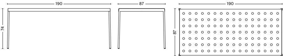
BALCONY TABLE Length 190 cm Width 87 cm Heigth 74 cm
