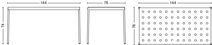
BALCONY TABLE Length 144 cm Width 76 cm Heigth 74 cm
