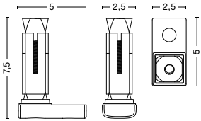
FIXATION BRACKET FOR TABLES Width 5 cm Depth 2,5 cm Height 7,5 cm
