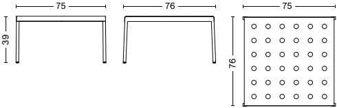
BALCONY LOW TABLE | SQUARE Length 75 cm Width 76 cm Heigth 39 cm
